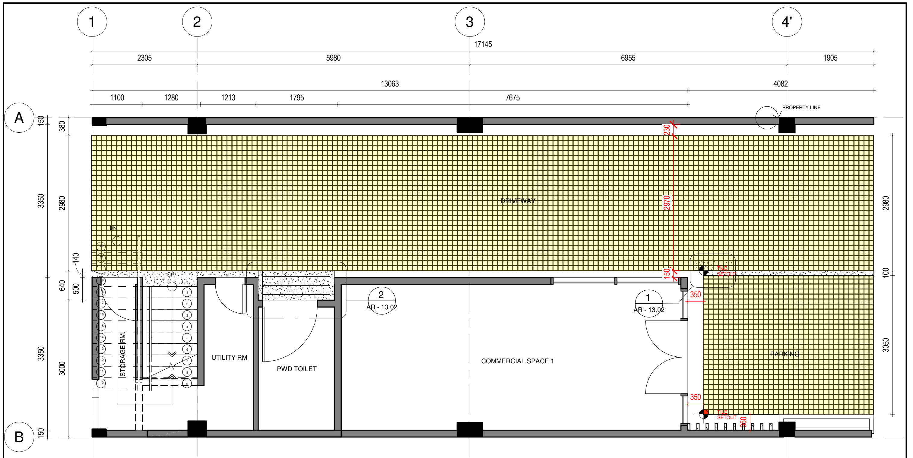
1 GROUND FLOOR FLOOR TILE LAYOUT AR - 13.01 SCALE 1 : 50 MTS
