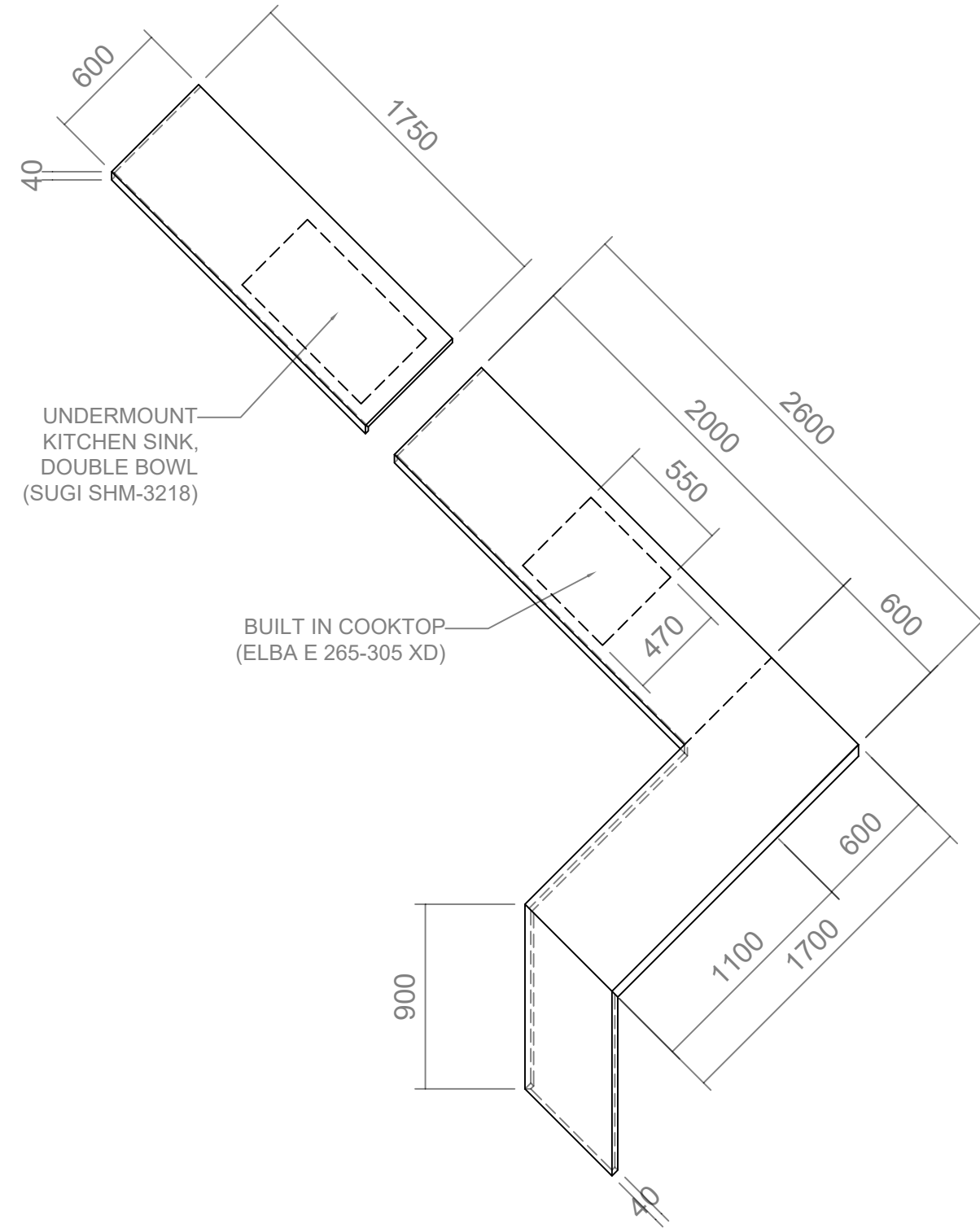
18MM THK COUNTERTOP WITH MITERED EDGE
