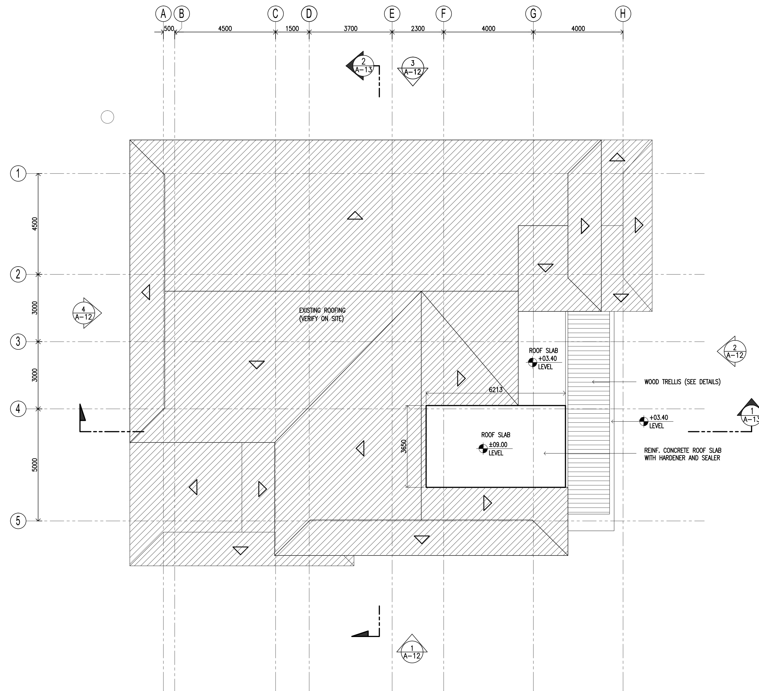
1 PROPOSED ROOF PLAN A-05 SCALE 1:100M
