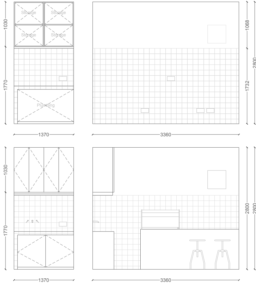
Altitud Coffee Space Preparation Area Elevation
