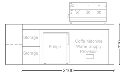
Altitud Coffee Space Bar Counter Working Drawing
