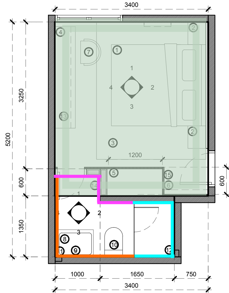
1 ID-1 MAJID'S BEDROOM + ENSUITE FLOOR + FURNITURE LAYOUT SCALE 1: 50 MTS.
