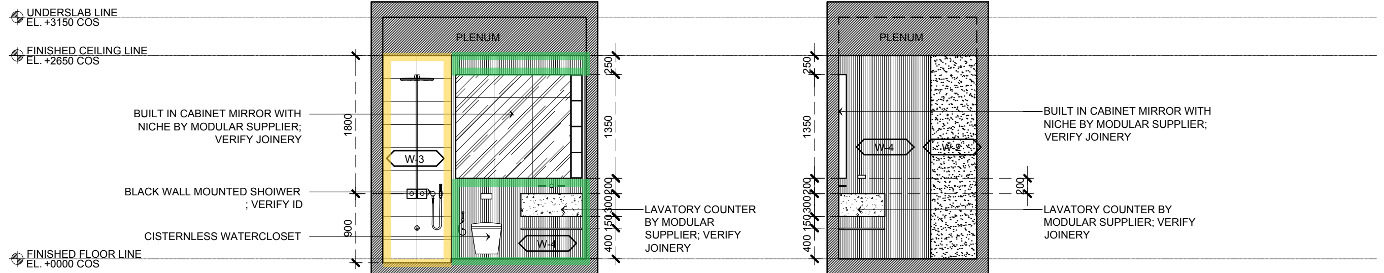
3 D-3 MAJID'S ENSUITE WALL ELEVATION - 3 SCALE 1:50MTS
