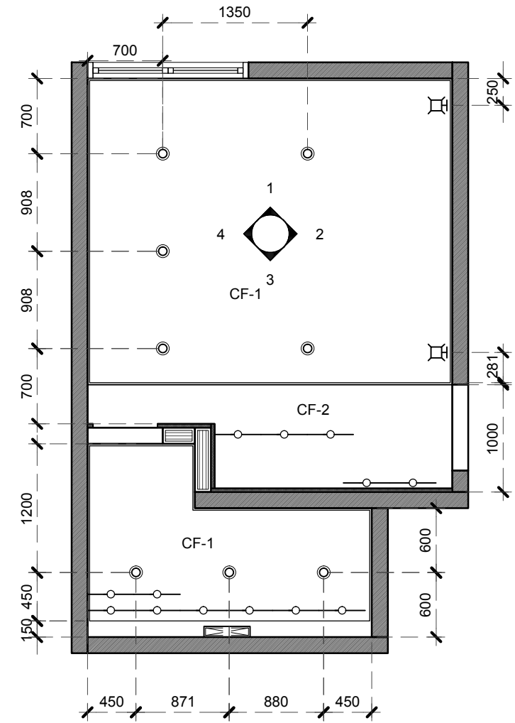
2 ID-1 MAJID'S BEDROOM + ENSUITE REFLECTED CEILING LAYOUT SCALE 1: 50 MTS.
